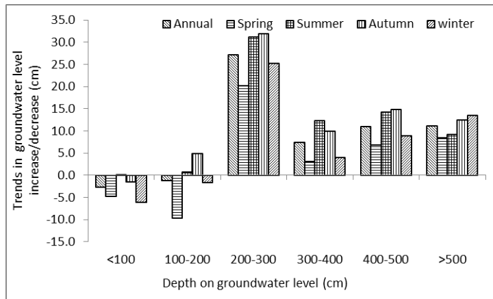
Fig. 2. Trends of groundwater level by depth of wells, in Moldavian Plain
