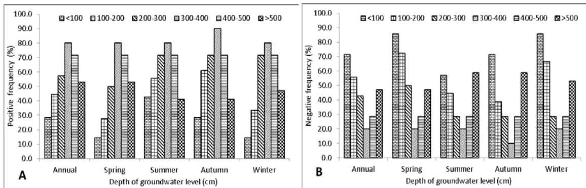
Fig. 3. Frequency of positive (A) and negative (B) slopes of the HL in Moldavian Plain
