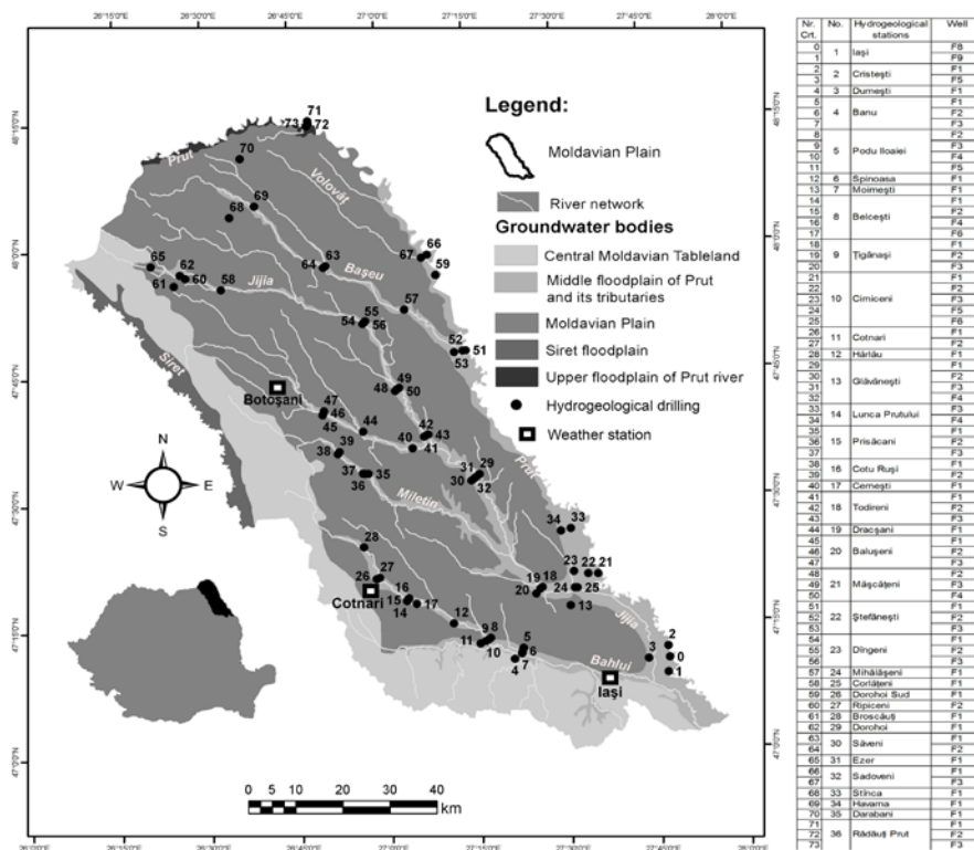
Fig. 1. The underground water bodies, weather stations and hydro-geological wells in Moldavian Plain
