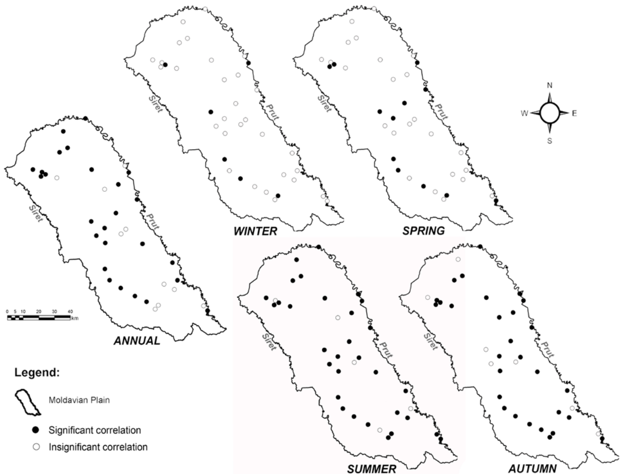
Fig. 4. Correlation between precipitation and hydrostatic level in Moldavian Plain
